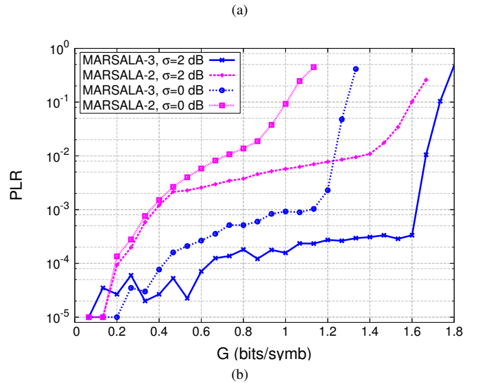
Fig. 4: Comparison between MARSALA-2 and MARSALA-3 with equi-powered packets and lognormally distributed packets power. QPSK modulation, DVB-RCS2 turbo code R = 1/3 , E_s/N_0 = 10 dB. (a) Throughput. (b) PLR.
