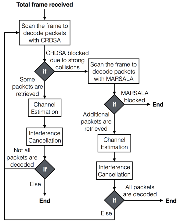
Fig. 1: Processing scheme for each frame at the receiver side, with combination of CRDSA and MARSALA.
