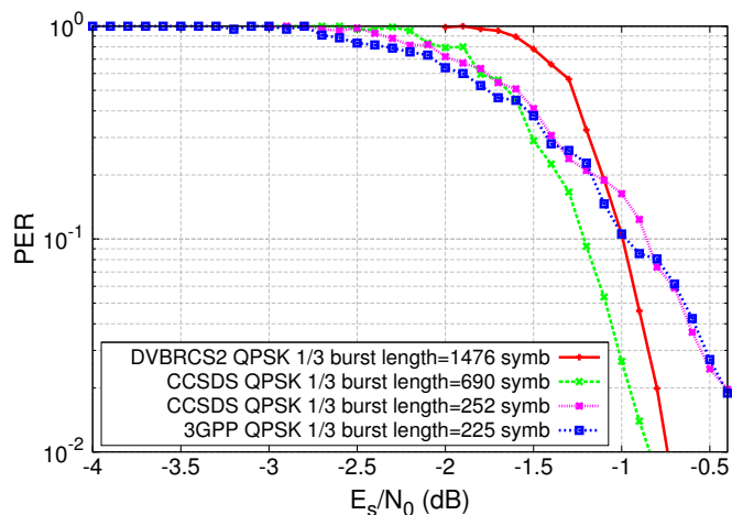
Fig. 7: PER vs. E_s/N_0 for 3GPP, DBB-RCS 2 and CCSDS turbo codes. QPSK modulation with code rate R = 1/3 .
