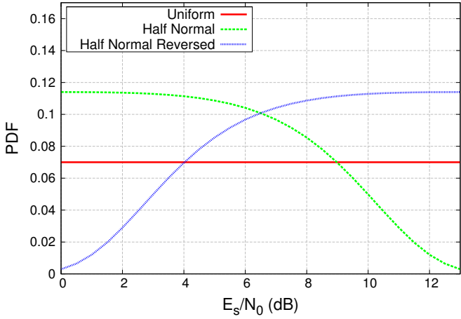
Fig. 5: PDFs proposed for packets power in MARSALA-3.
