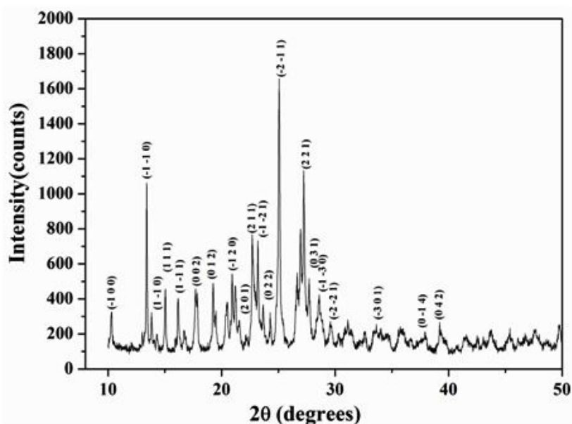
Fig. 2. Indexed powder XRD pattern of PNQI.
