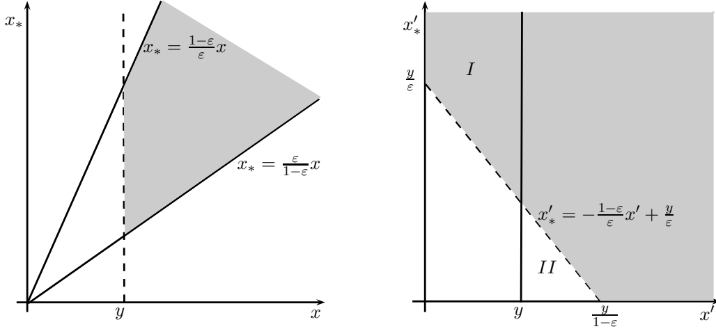
FIGURE 1. Change of variables and integration areas I and II
