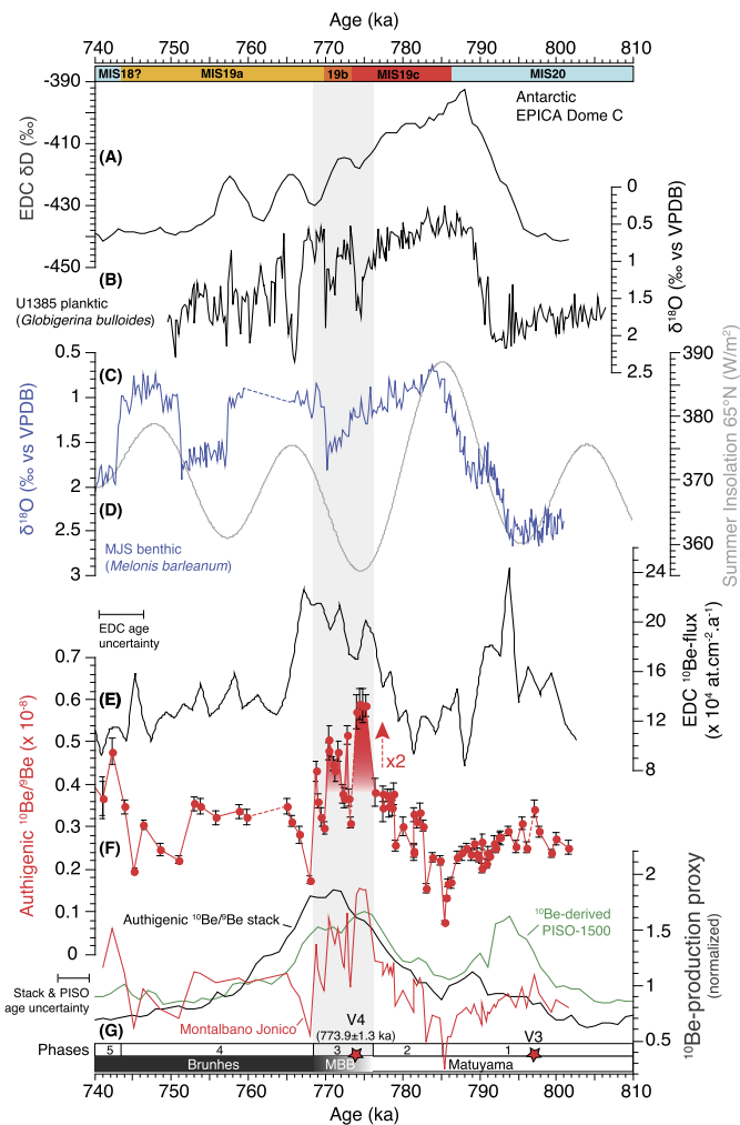
Fig. 6. Chronology of the MBB. Authigenic ^{10}\text{Be}/^9\text{Be} ratio (F, red line) and benthic \delta^{18}\text{O} Melonis barleauum record (C, blue line) from the Ideale section are compared to references. (A) \delta\text{D}_{\text{ice}} record and (E) ^{10}\text{Be} -fluxes from the Epica Dome C plotted according to the AICC2012 age model (Jouzel et al., 2007; Raisbeck et al., 2006; Bazin et al., 2013). (B) North Atlantic planktic \delta^{18}\text{O} record of Globigerina bulloides from U1385 (Sánchez Goñi et al., 2016) plotted on the orbital tuned time scale (Hodell et al., 2015). (D) 65^\circ\text{N} summer insolation (Laskar et al., 2004). (G) Equatorial authigenic ^{10}\text{Be}/^9\text{Be} ratio normalized stack (black; Simon et al., 2016a), authigenic ^{10}\text{Be}/^9\text{Be} ratio normalized record from Montalbano Jonico (red) and ^{10}\text{Be} -production computed from the PISO-1500 marine sediment RPI stack (green; Channell et al., 2009) using the theoretical ^{10}\text{Be} production model of Masarik and Beer (2009). Marine isotopic substages are from this study. The MBB time interval highlighted by grey bar is inferred from the authigenic ^{10}\text{Be}/^9\text{Be} ratio peak and geometrically centered at: \sim 772.5 ka ( 776\text{--}768.5 ka). (For interpretation of the references to color in this figure legend, the reader is referred to the web version of this article.)
