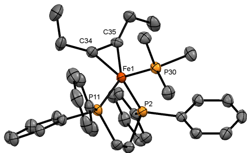
Figure 5. Thermal ellipsoid representation (at 50% probability) of complex 9 . H atoms are not shown for clarity. Selected bond length (Å) and angles (°): P11-Fe1-P2 86.76(5); P11-Fe1 2.1501(14); P2-Fe1 2.136(14); P30-Fe1 2.150(14); Fe1-C34 1.874(5); Fe1-C35 1.860(5); C34-C35 1.303(6).
