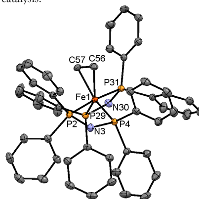
Figure 3. Thermal ellipsoid representation (at 50% probability) of complex 7 . H atoms are not shown for clarity. Selected bond length (Å) and angles (°): P2-Fe1-P4 71.70(2); P29-Fe1-P31 71.78(2); C57-C56 1.423(3); C56-Fe1 2.069(2); C57-Fe1 2.050(2); P4-Fe1 2.189(6); P2-Fe1 2.209(6); P31-Fe1 2.198(6); P29-Fe1 2.175(6).
