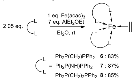
Scheme 2. Synthetic route to complexes 6-8.
