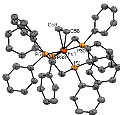
Figure 4. Thermal ellipsoid representation (at 50% probability) of complex 8 (50% probability displacement ellipsoids). H atoms are not shown for clarity. Selected bond length (Å) and angles (°): P2-Fe1-P5 84.35(8); P33-Fe1-P30 83.72(8); C59-C58 1.441(11); C59-Fe1 2.082(8); C58-Fe1 2.099(7); P5-Fe1 2.229(2); P2-Fe1 2.238(2); P33-Fe1 2.214(2); P30-Fe1 2.210(2).
