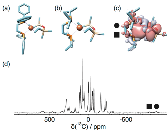
Figure 2. (a) X-ray structure of 1 (H atoms not shown for clarity). (b) DFT-optimized structure of 5 . (c) Visualization of positive (blue) and negative (red) isosurfaces of spin density distribution in 5 (for \pm 0.0002 a.u. isovalues). (d) ^{13}\text{C} PNMR spectrum of 5 . The two \text{CH}_2 carbons and their signals are labeled with a circle and a square in panels (c-d).
