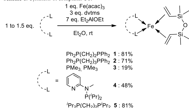
Scheme 1. Synthesis of complexes 1-5.
