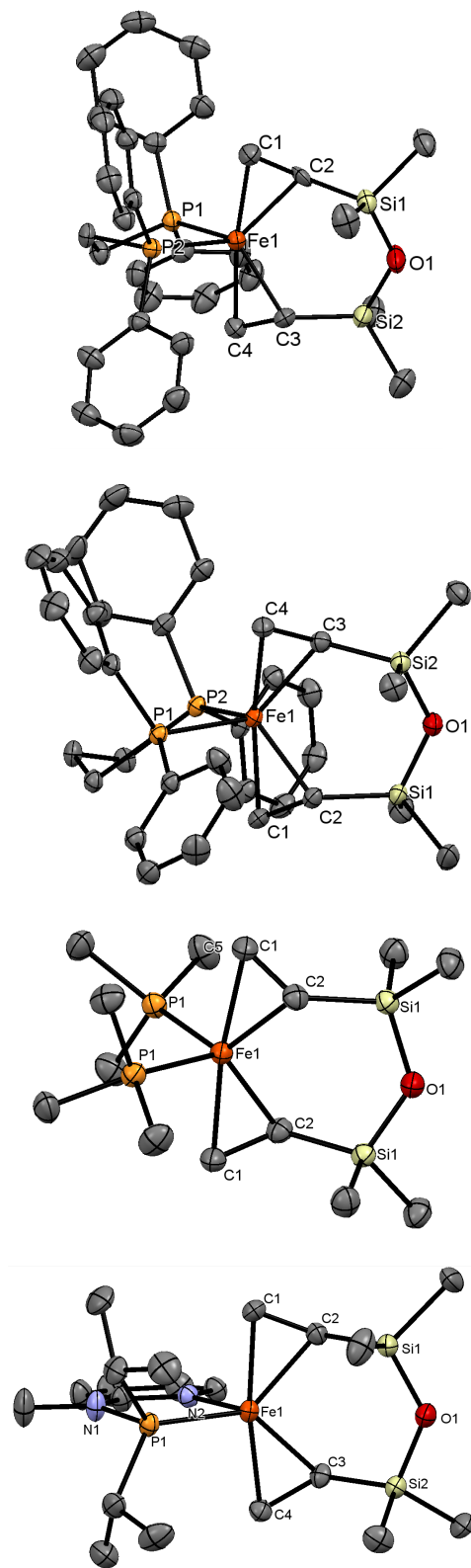
Figure 1. Thermal ellipsoid representation (at 50% probability) of complexes (from top to bottom) 1 , 2 , 3 and 4 ; H atoms are not shown for clarity. Selected bond lengths (Å) and angles ( ^\circ ): For 1 : P1-Fe1-P2 84.75(3); P1-Fe1 2.302(10); P2-Fe1 2.316(10); C3-C4 1.419(5); C1-C2 1.409(5); for 2 : P1-Fe1-P2 91.37(2); P1-Fe1 2.291(6); P2-Fe1 2.335(6); C3-C4 1.418(3); C1-C2 1.415(3); for 3 : P1-Fe1-P1
