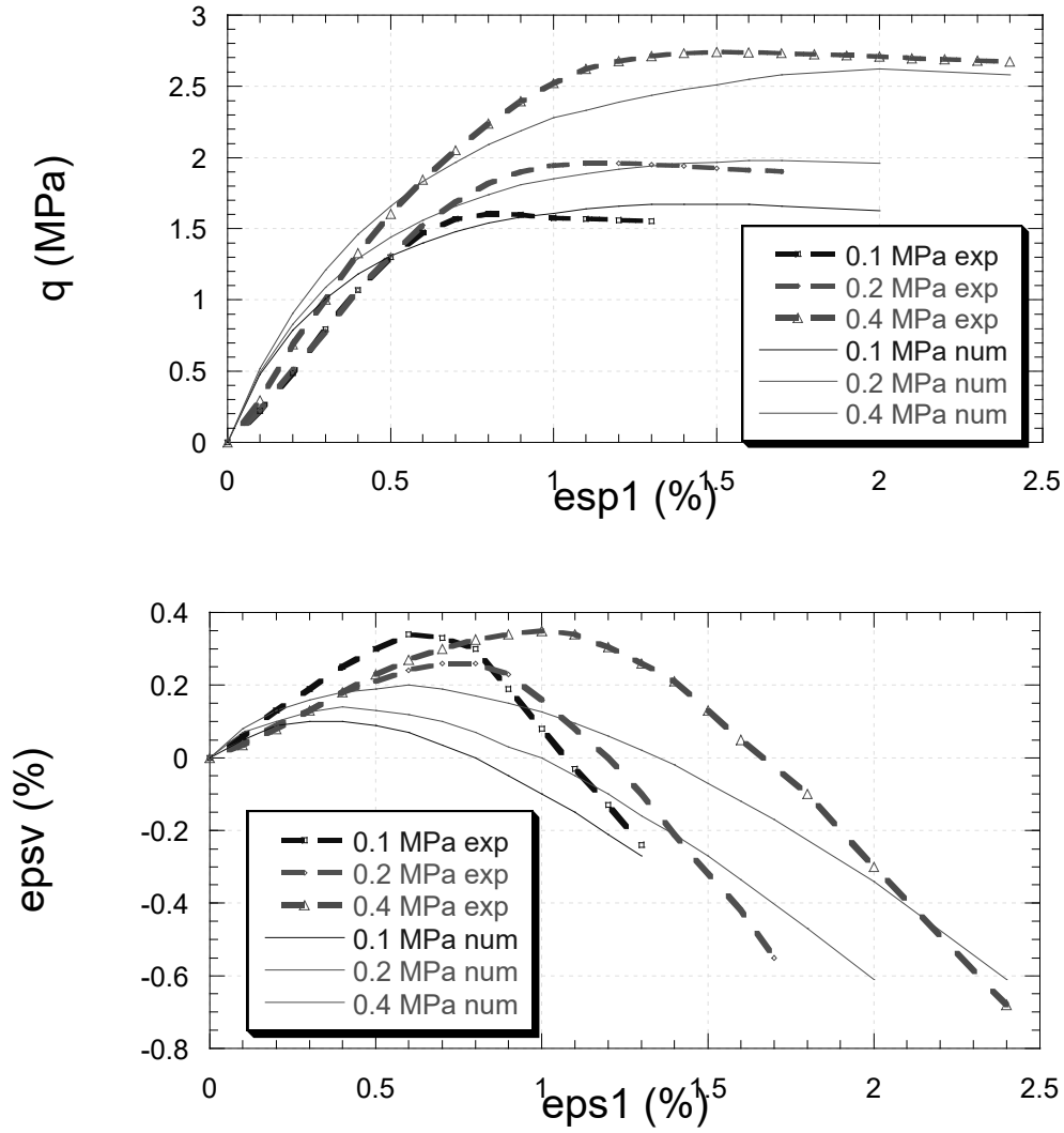
Fig. 2. Grouted Fontainebleau Sand by Intra-J C/W = 0.175
