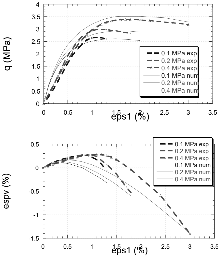
Fig. 3. Grouted Fontainebleau Sand by Intra-J C/W = 0.23
