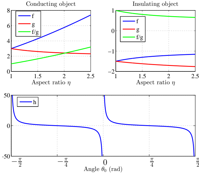
Fig. 9: Functions f , g and f/g for a conducting object (top left) and an insulating object (top right) over the interval [1; 2.5] . Function h over the interval [-\frac{\pi}{2}; \frac{\pi}{2}] (bottom).
