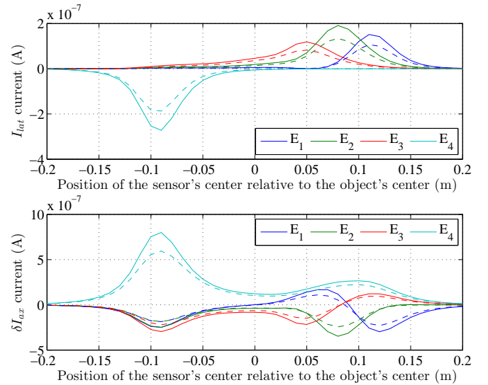
Fig. 4: Currents I_{\text{lat}} (top) and \delta I_{\text{ax}} (bottom) for a straight line motion of the sensor, with constant polarization vector U = (0 \ 0 \ 0 \ 1)^T , going past the object numbered 5 in table I. Solid lines : BEM currents. Dashed lines : currents calculated with the analytical model.
