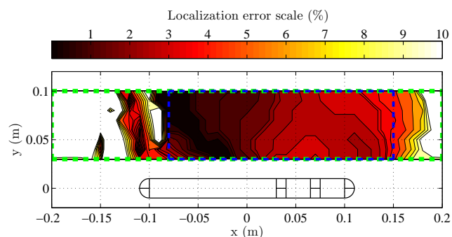
Fig. 6: MUSIC localization error map in percentage of sensor length (22cm) for a 1cm radius conducting sphere placed inside the green dashed line delimited area. Blue dotted line roughly defines an area in which the error is less than 5%.
