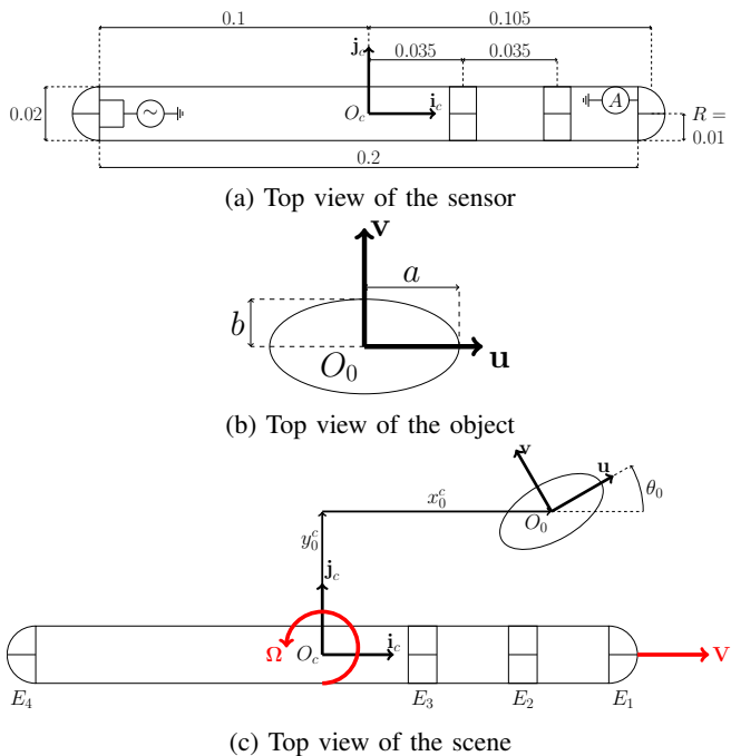
Fig. 1: (a) The sensor with the polarization and measurement schematic and dimensions in meters. R denotes the sensor radius. (b) The ellipsoid and its related local frame ( O_o , \mathbf{u} , \mathbf{v} ). O_o coincides with the geometrical center of the object. Vectors \mathbf{u} and \mathbf{v} are aligned with the semi-major axis ( a ), and the semi-minor axis ( b ), respectively. (c) The sensor, the object and their respective frames. The coordinates of the geometrical center of the object are denoted (x_0^c, y_0^c) in the sensor frame. Its orientation relative to the sensor axis is \theta_0 . Vector \mathbf{V} is the longitudinal velocity and vector \mathbf{\Omega} is the rotation velocity about the vertical axis. The macro-electrodes are numbered from E_1 to E_4
