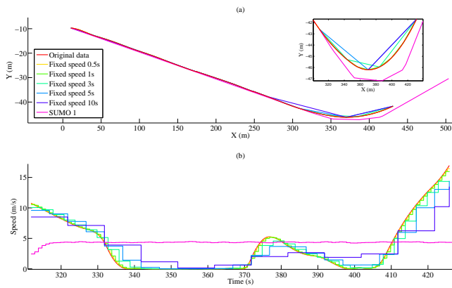
Fig. 8. (a) Position and (b) speed of node 10 group 2, over time for different models of mobility
