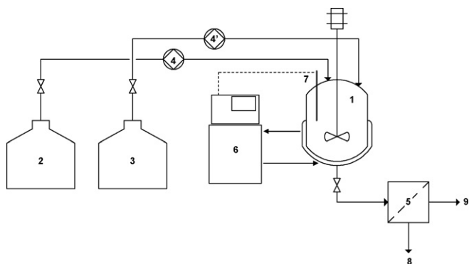
Fig. 1. Experimental set-up of the removing of ethanolic insoluble compounds contained in sugar beet vinasse (1: 5 L double-jacketed reactor; 2: sugar beet vinasse tank; 3: ethanol tank; 4, 4': peristaltic pumps; 5: filter; 6: thermo-regulator; 7: thermometric probe; 8: filtrate; 9: precipitate).
