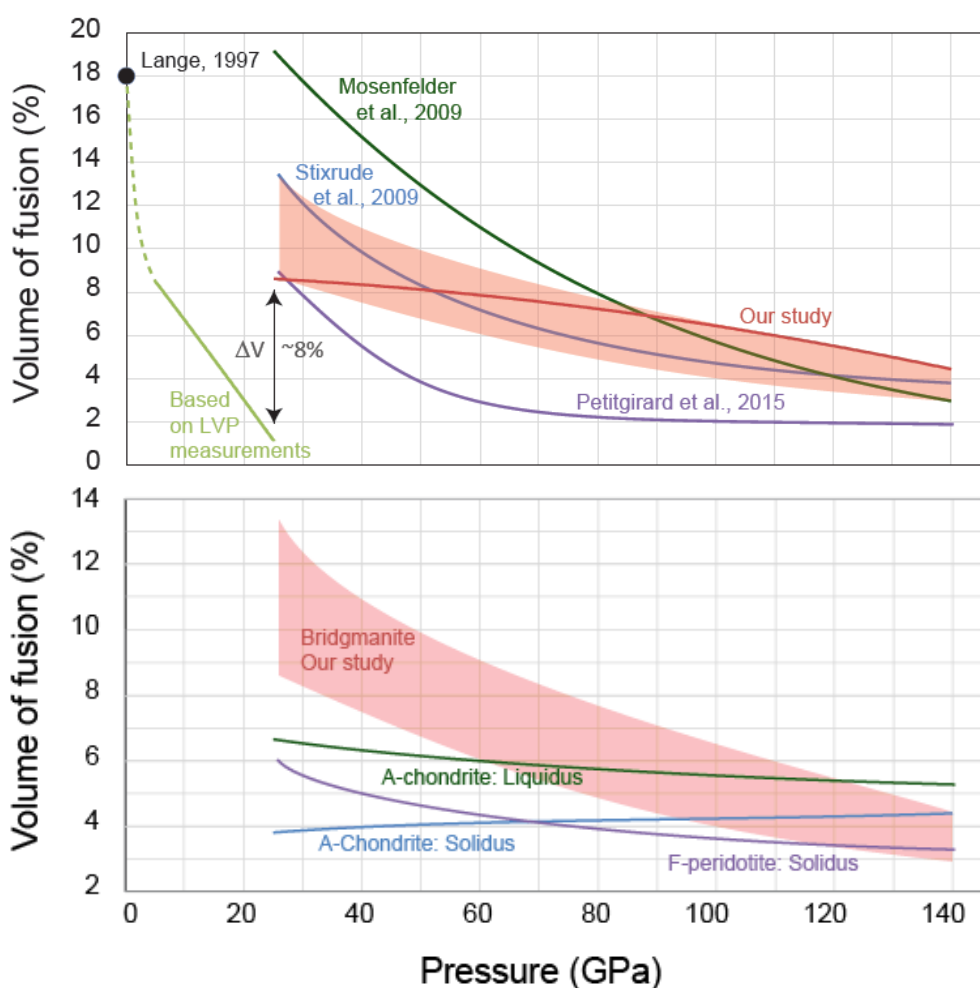
Figure 2: (a) Volume of melting ( \Delta V_m = V_{\text{melt}} - V_{\text{Solid}}/V_{Bg} , where V_{Bg} is volume of Bridgmanite) derived from the melting curve of Bg (Figure 1) with various (Mg,Fe)(Si,Al) \text{O}_3 compositions. We also report the value of 18% measured for pure \text{MgSiO}_3 at 1 bar (Lange, 1997) and \Delta V_m/V_{Bg} recalculated from density measurements of \text{MgSiO}_3 -glass in a DAC (Petitgirard et al., 2015). Shaded pink region is the most probable range of mantle \Delta V_m/V_{Bg} values. (b) \Delta V_m derived from the solidus and/or liquidus profiles of the A-chondritic (Andrault et al., 2011) and F-peridotitic (Fiquet et al., 2010) models of mantle melting. \Delta V_m is calculated using the Clapeyron relation. Calculation of \Delta V_m/V_{Bg} along solidus and liquidus profiles assume an ideal mixing model to estimate the melt entropy (see text).
