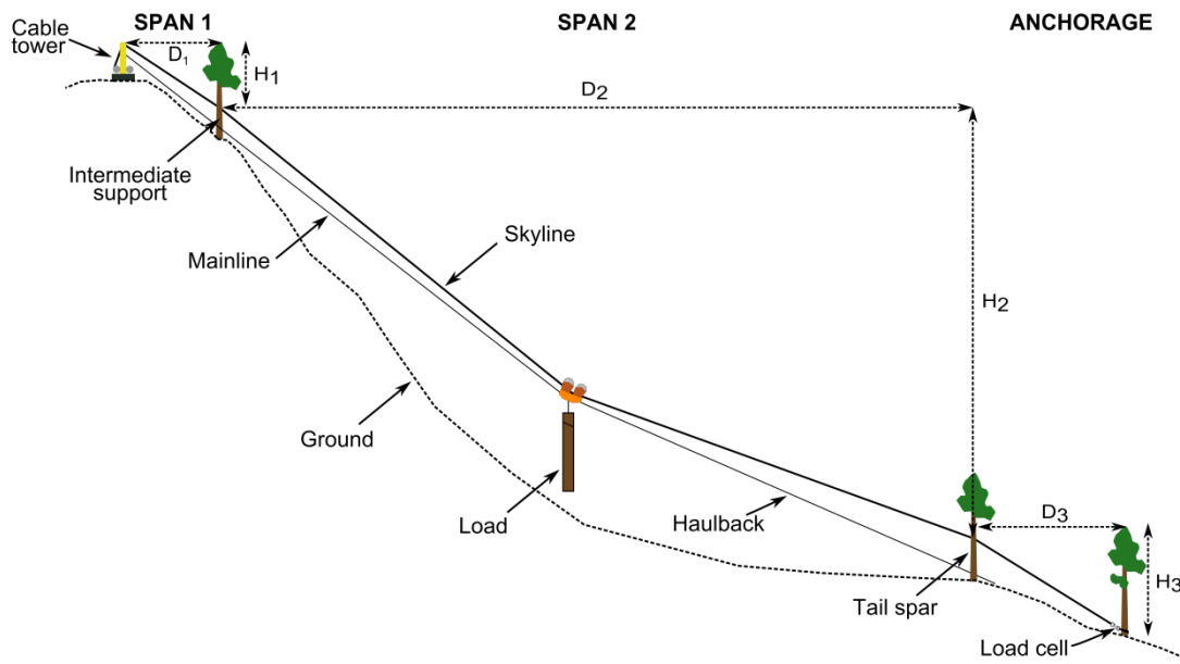
Annex 3 Scheme of the real cable yarding operation followed. Measurements concern the situation when the load is located on SPAN 2 to ensure a full suspension of the log.
