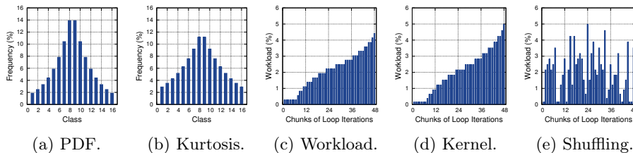
Figure 1: Impact of performance factors in the application's workload.
