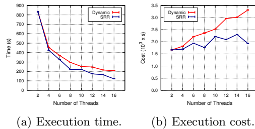
Figure 4: Results for strong scaling runs on the LavaMD kernel.
