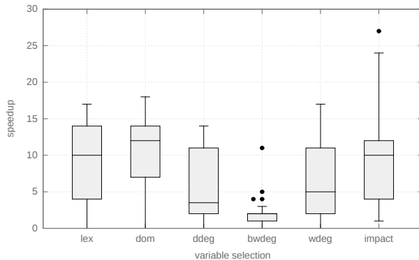
Figure 5: Speedups of the variable selection heuristics (Choco2, data center, w = 16 ).
