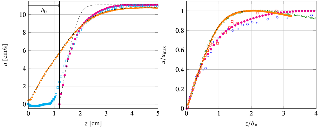
Figure 6: Velocity profiles near the rough plate at Ra = 4.66 \times 10^9 , in a groove (full orange triangles), on the top of a roughness element (full magenta circles) and inside a notch (cyan squares, full symbols obtained with the acquisition inside the notch, open symbols with the acquisition above the notch, away from the plate). The black dashed lines are the theoretical Prandtl-Blasius profiles. Left: raw profiles where the origin z = 0 is the bottom of the roughness elements. Right: non-dimensional profiles compared with experimental data obtained in smooth cells at Ra = 7.48 \times 10^{11} from du Puits et al. (2007) (open blue circles), at Ra = 3 \times 10^9 from Li et al. (2012) (open red squares) and at Ra = 5.3 \times 10^9 from Sun et al. (2008) (open green triangles).
