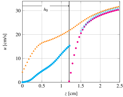
Figure 7: Velocity profiles near the rough plate at Ra = 4.04 \times 10^{10} , in a groove (full orange triangles), on the top of a roughness element (full magenta circles) and inside a notch (full cyan squares: acquisition of the low velocities, open cyan squares: acquisition of the fast velocities).
