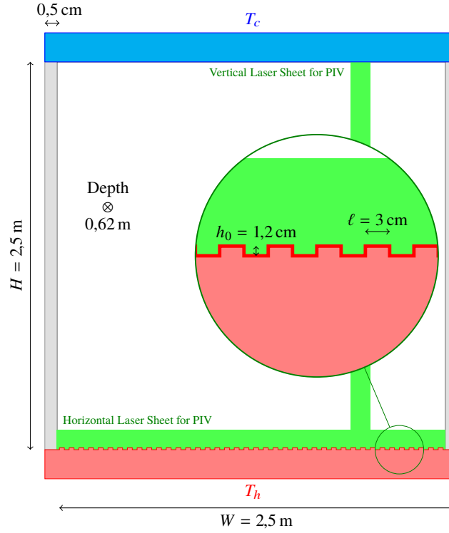
Figure 1: Sketch of the convection cell. The green surfaces represent the laser sheets, either vertical for PIV in the groove and on the obstacle, or horizontal for PIV inside the notch.
