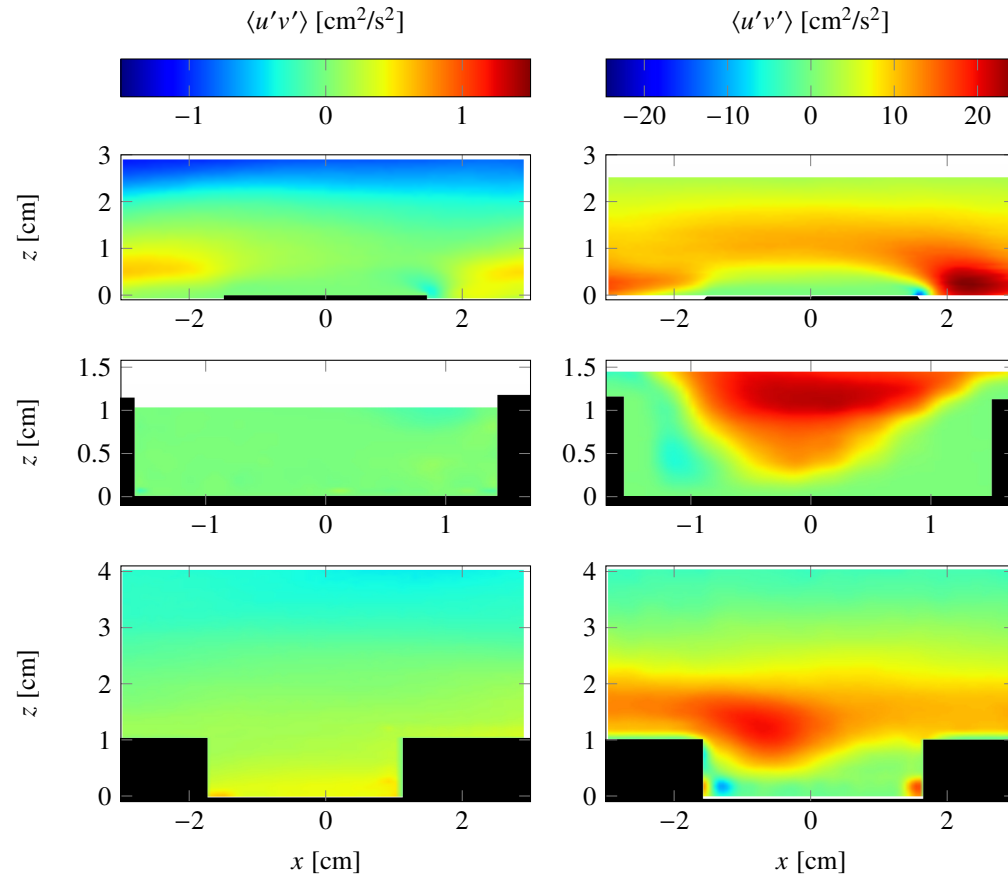
Figure 8: Reynolds tensor at Ra = 4.66 \times 10^9 (left) and Ra = 4.04 \times 10^{10} (right). From top to bottom: on top of an obstacle, inside a notch, in a groove. The color code is given for one Rayleigh number, identical for the three locations. The first column yields U^* = 0.77 cm/s at Ra = 4.66 \times 10^9 ; the second column U^* = 4.96 cm/s at Ra = 4.04 \times 10^{10} .
