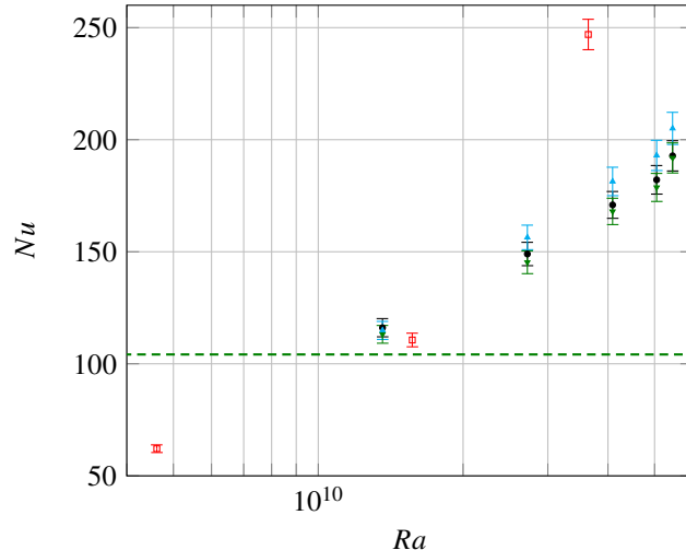
Figure 3: Non-dimensional local heat-flux measurements at x = 60 cm inside the rough cell (red open squares). The error bars represents the 5.5% uncertainty of the commercial heat-flux sensors on the dimensionless heat-flux. The results from Kaiser (2015) inside a smooth cell is shown for reference: whole-plate heat-flux measurements from IR camera (black circles) with an uncertainty of 7%, heat-flux averaged on 3\text{ cm} \times 3\text{ cm} area at x = 60 cm (down-pointing green triangles) and at x = 190 cm (up-pointing cyan triangles). The horizontal dashed line indicates the transition Nusselt number, Nu_c = H/(2h_0) , above which a heat transfer enhancement is expected.
