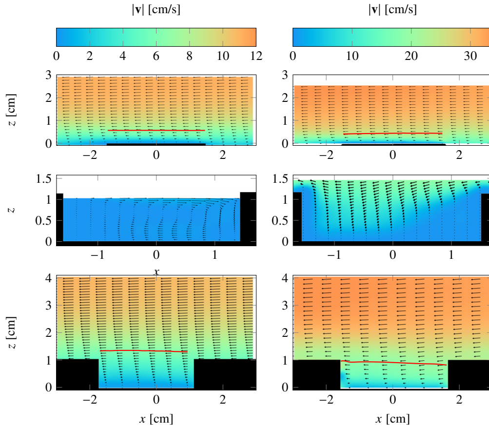
Figure 5: Mean velocity fields at Ra = 4.66 \times 10^9 (left) and Ra = 4.04 \times 10^{10} (right). From top to bottom: on top of an obstacle, inside a notch, in a groove. The color code is given for one Rayleigh number, identical for the three locations. The scale of the arrows is arbitrary and differs from one plot to another to allow better visualization of the flow. The solid red line is the velocity displacement thickness, \delta_{\text{displacement}} (see Eq. 8).
