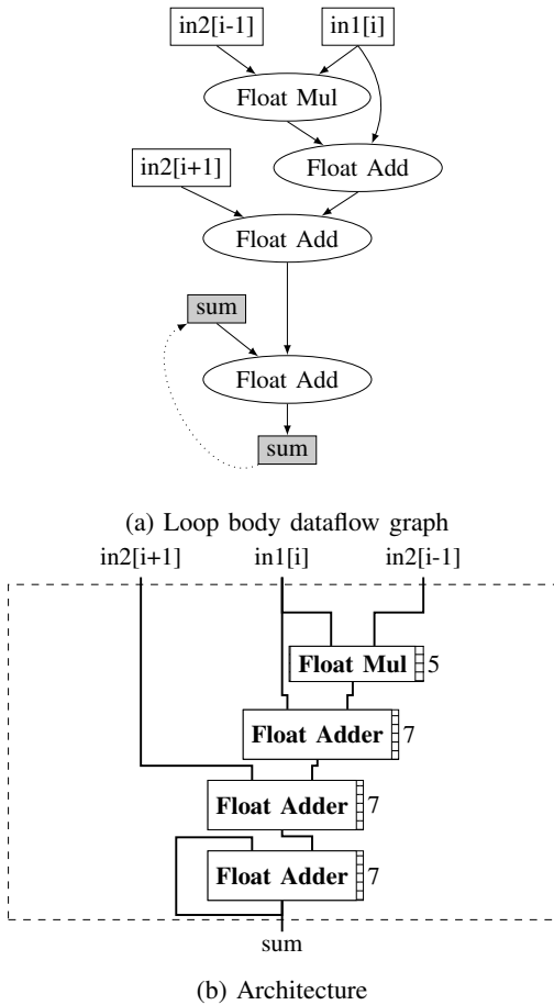
Figure 4: DFG of the loop body from Listing 5 (top) and its corresponding architecture (bottom). Keywords float mul and float add correspond to floating-point multipliers and adds respectively
