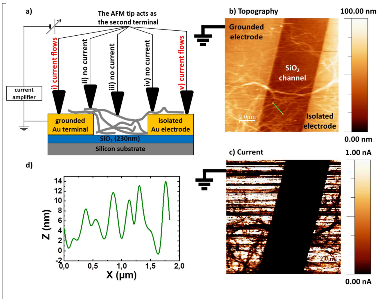
Figure 2 | C) C-AFM measurements performed on hybrid fibers deposited in-between gold electrodes.
