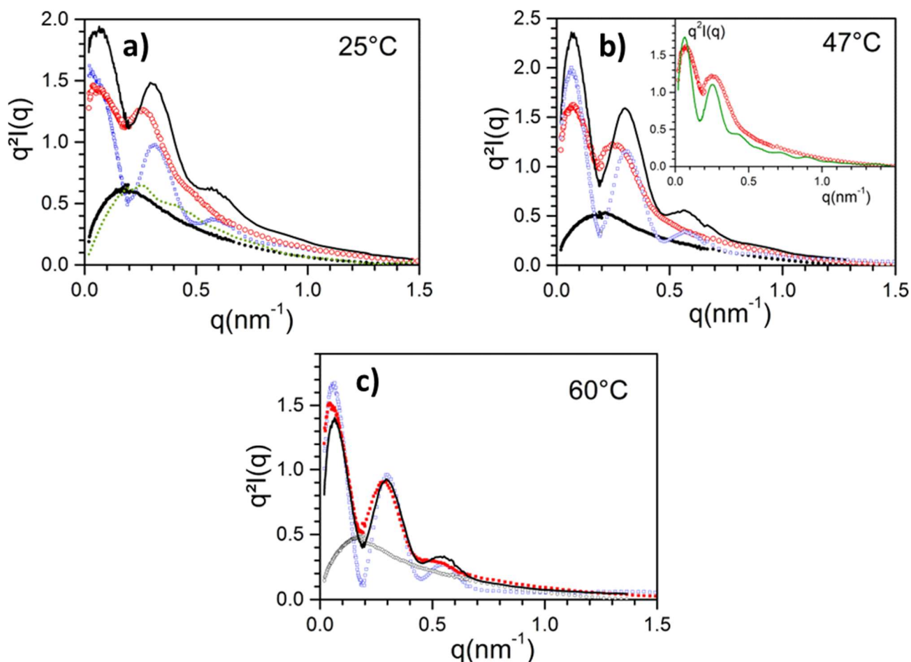
Figure 3 | Small-angle scattering curves plotted by means of a Kratky-plot ( q^2I(q) vs q ) for the binary system P3BT/trans-decahydronaphthalene gels, C_{\text{P3BT}} = 0.01 \text{ g/cm}^3 (black dots); the binary system BHPB-10/trans-decahydronaphthalene gels, C_{\text{BHPB-10}} = 0.01 \text{ g/cm}^3 (blue open squares); the ternary system P3BT/BHPB-10/trans-decahydronaphthalene, C_{\text{BHPB-10}} = 0.01 \text{ g/cm}^3 + C_{\text{P3BT}} = 0.01 \text{ g/cm}^3 (red open circles); the solid curve stands for the sum of the intensities of each binary system, except at 60^\circ\text{C} where it represents 70% of this sum. a) T = 25^\circ\text{C} b) T = 47^\circ\text{C} , inset shows the best fit in solid green curve (see text for details) and c) T = 60^\circ\text{C} .
