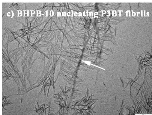
Figure 1: The preparation protocol, top; bottom TEM pictures obtained on: a) purified P3BT fibrils prepared in trans-decahydronaphthalene at room temperature; b) BHPB-10 ringlets produced by quenching at 0°C solutions in trans-decahydronaphthalene; c) P3BT fibrils nucleated onto BHPB-10 nanotubes (arrow) by cooling a homogeneous mixture ( 0.05 \times 10^2 \text{g/cm}^3 \text{P3BT} + 0.01 \times 10^2 \text{g/cm}^3 \text{BHPB-10} ); d) hybrid system obtained by mixing P3BT fibrils grown beforehand with BHPB-10 SOL at 60°C and then quench to 0°C. White scale bar= 200 nm. Note that the systems are diluted to 10 to 100 times to allow for TEM observations.
