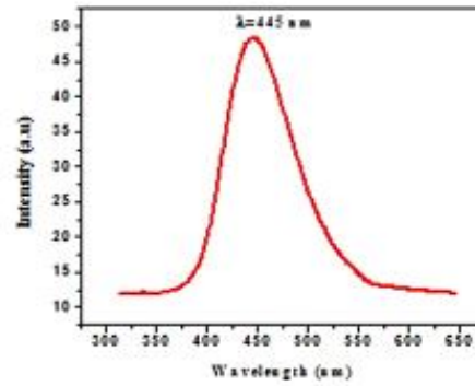
Fig. 7. PL spectrum of GCHBS.
