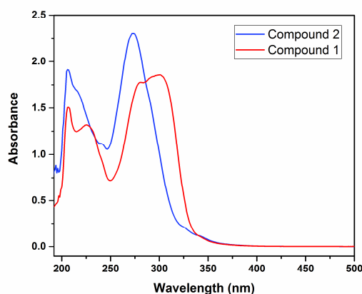
Fig. 2. UV Vis spectra of compound 1 and 2.
