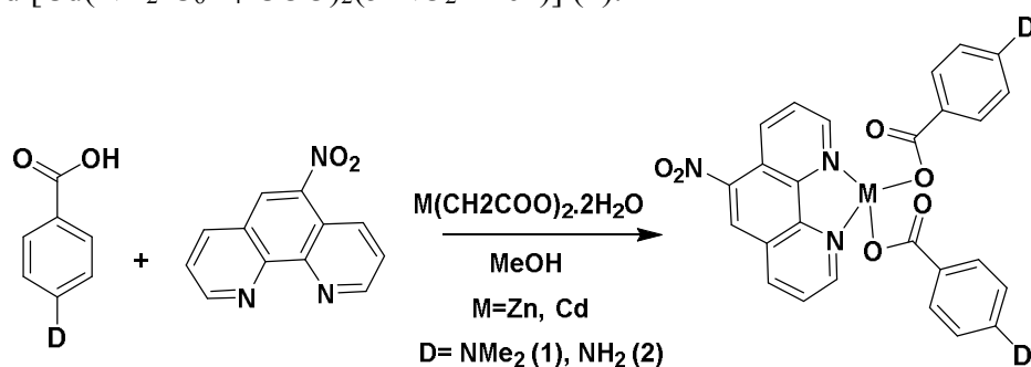
Fig. 1. Scheme of Synthesis.
