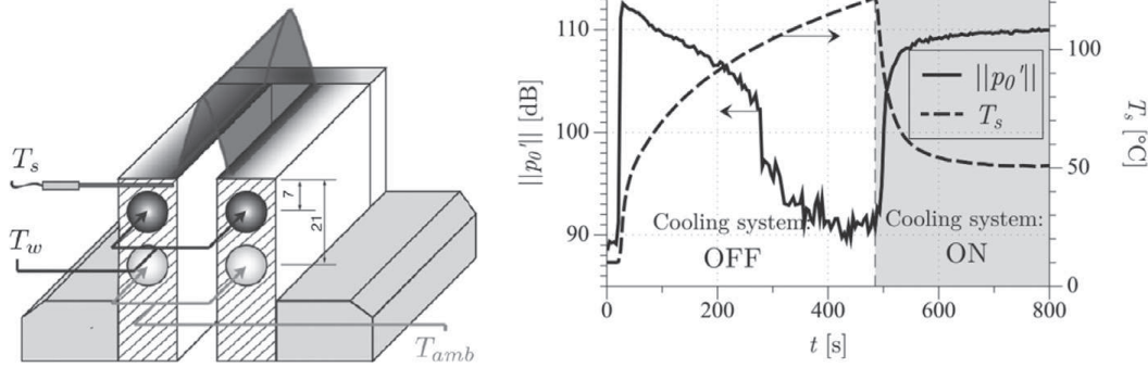
Fig. 10. Demonstrating the effects of flame holder temperature on the stability of a laminar premixed Bunsen flame [113]. Left: a Bunsen flame stabilized on a water-cooled slot. Right: evolution of pressure oscillations and slot wall temperature versus time. The cooling system is started at t = 490 s.
