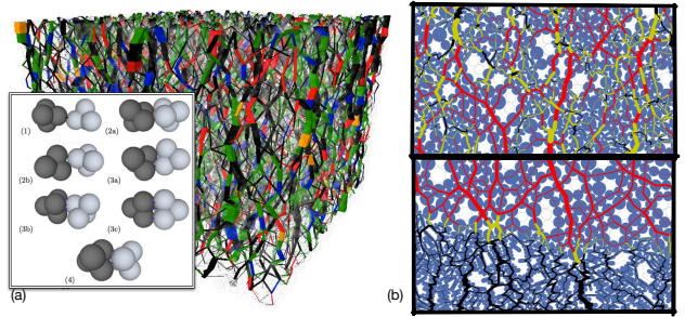
Figure 4. Snapshot of normal forces in (a) packing composed of non-convex particles (here \eta = 0.6 ), and (b) packings composed of mixture of two shape for homogeneous (up) and segregated (down) packings. The forces are plotted in different colors depending on contact types. The inset shows contacts type for non-convex aggregate whereas in mixture we can distinguish disks-disks, discs-elongated and elongated-elongated contacts.
