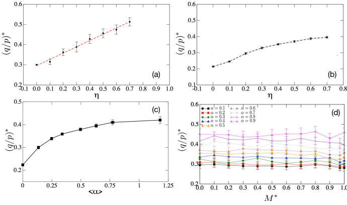
Figure 3. Normalized shear strength averaged in the steady state as a function of particle platyness/elongation (a), non-convexity (b), angularity (c), and as function of packing homogeneity for all values of mixture ratio (d).
