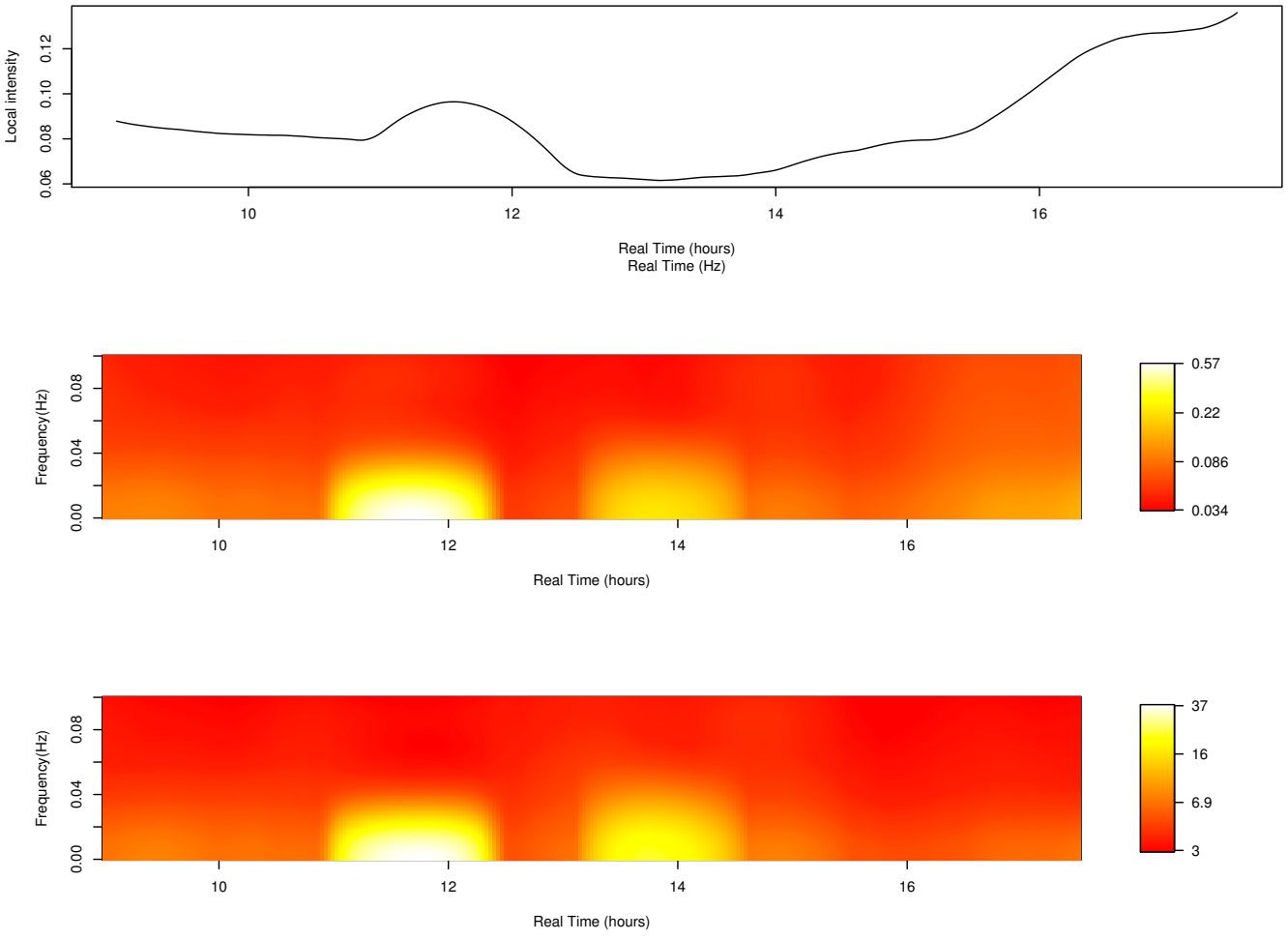
Figure 1: Averaged local mean density (top) and Bartlett spectrum, nonnormalized (middle) and Poisson-normalized (bottom), for ESSIPPA transaction data.
