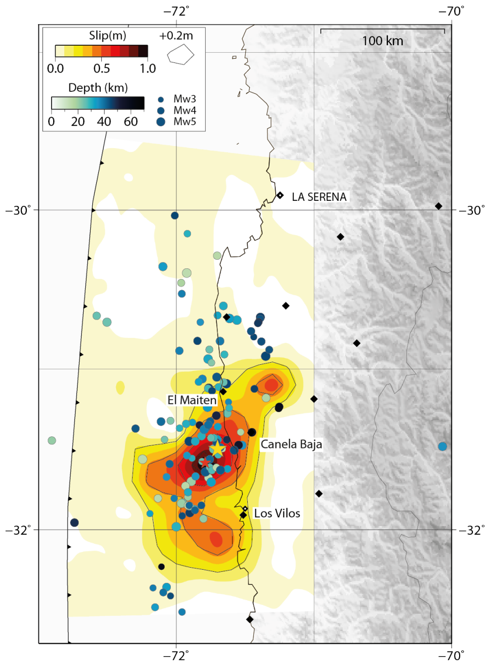
Fig. 6: Slip distribution of HF solution - daily solution. Slip distribution of the best fit model of the difference between the high rate and the daily coseismic static solutions corresponding to the main aftershock (epicenter depicted by the yellow star, CSN) plus postseismic deformation on the first hours after the main shock and the aftershock (epicenter depicted by the red star [Ruiz et al.,2016]). Dots represent aftershocks of M_w < 5 (CSN catalog), that occurred during the same period. Black diamonds depict the location of HR stations used. Estimated M_0 = 2.14 \times 10^{20} N.m ( M_w = 7.5 )
