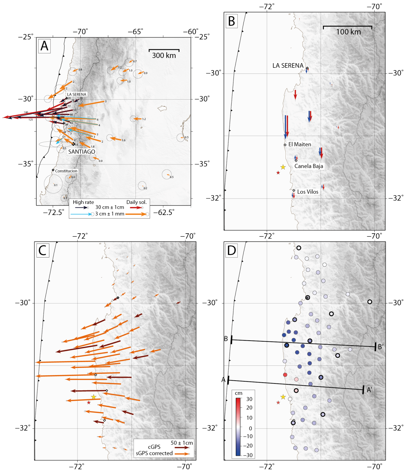
Fig. 2: Co-seismic static displacement field.
