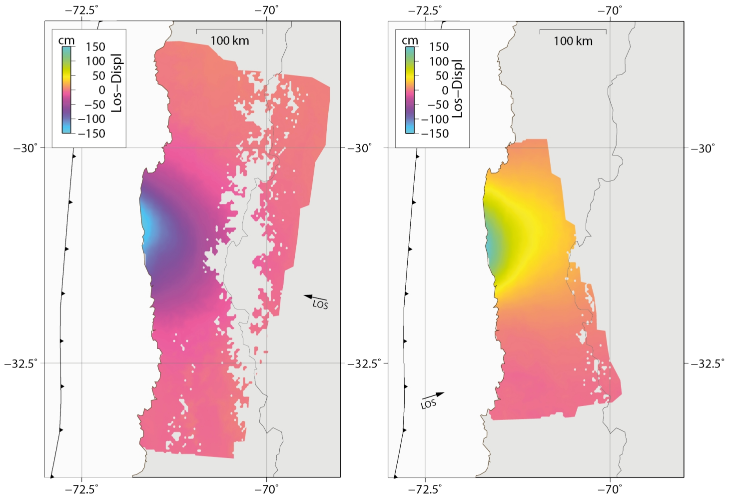
Fig. 3: Unwrapped InSAR data. Descending (left) and ascending (right) reconstructed unwrapped InSAR Sentinel-1 tracks). The LOS vector is indicated by the black arrow. Incidence angle increases from 30^\circ in near range to 46^\circ in far range.
