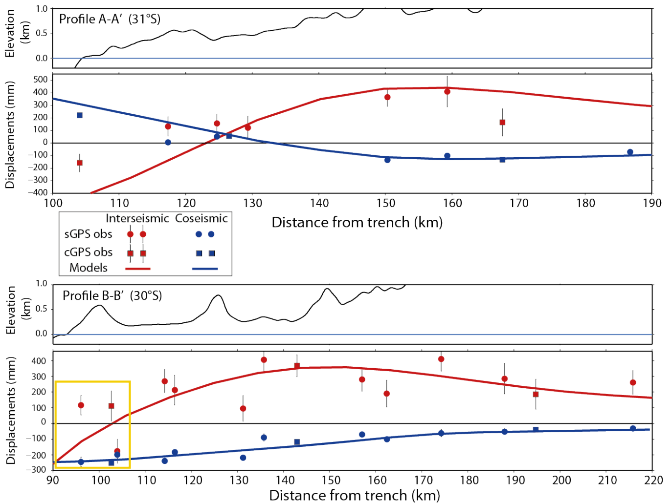
Fig. 8: Interplay between interseismic and coseismic deformation. Comparison of cumulated vertical interseismic displacements over 72 years measured (red dots) and modelled (red curve from Métois et al., 2016, models were mostly constrained on the horizontal interseismic deformation between 2004 and 2012 and are here extrapolated over 72 years, in mm) vs vertical coseismic displacements measured (blue dots) and modelled (blue curve), in mm. Profiles are represented on fig.2D. Topographic profiles are from ETOPO. (The yellow square highlights the area where the coseismic and interseismic models show both subsidence.)
