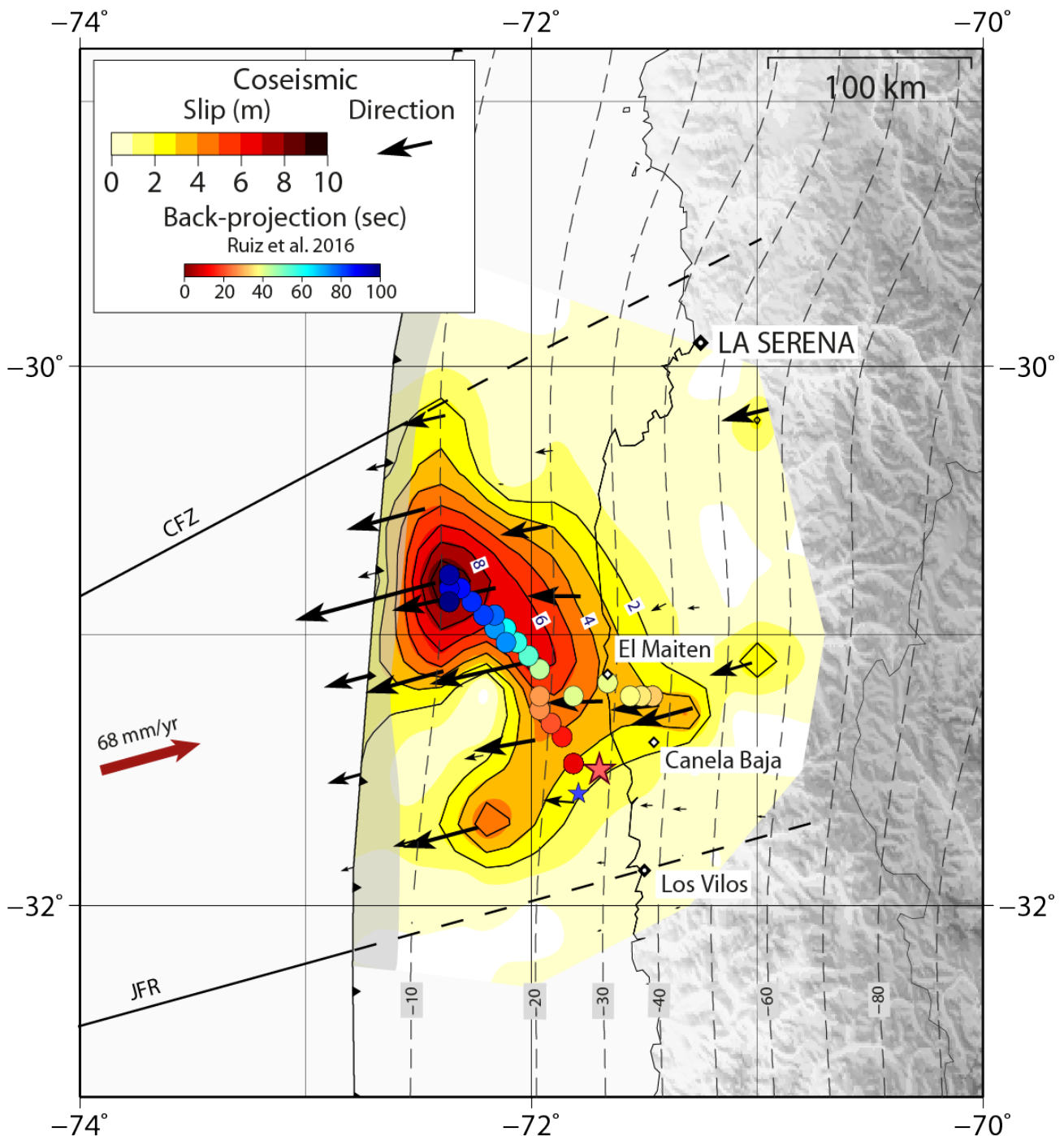
Fig. 4: Slip distribution of the preferred model of this study (red color scale), black arrows show slip direction of slip. Black lines represented the Challenger Fracture Zone [Contreras et al., 2011] and the Juan Fernandez Ridge [Yáñez et al., 2001], extrapolated along the subduction interface, slab isodepths from Slab1.0 [Hayes et al., 2012]. The Nazca/South-America convergence rate and direction are represented by the red arrow.
