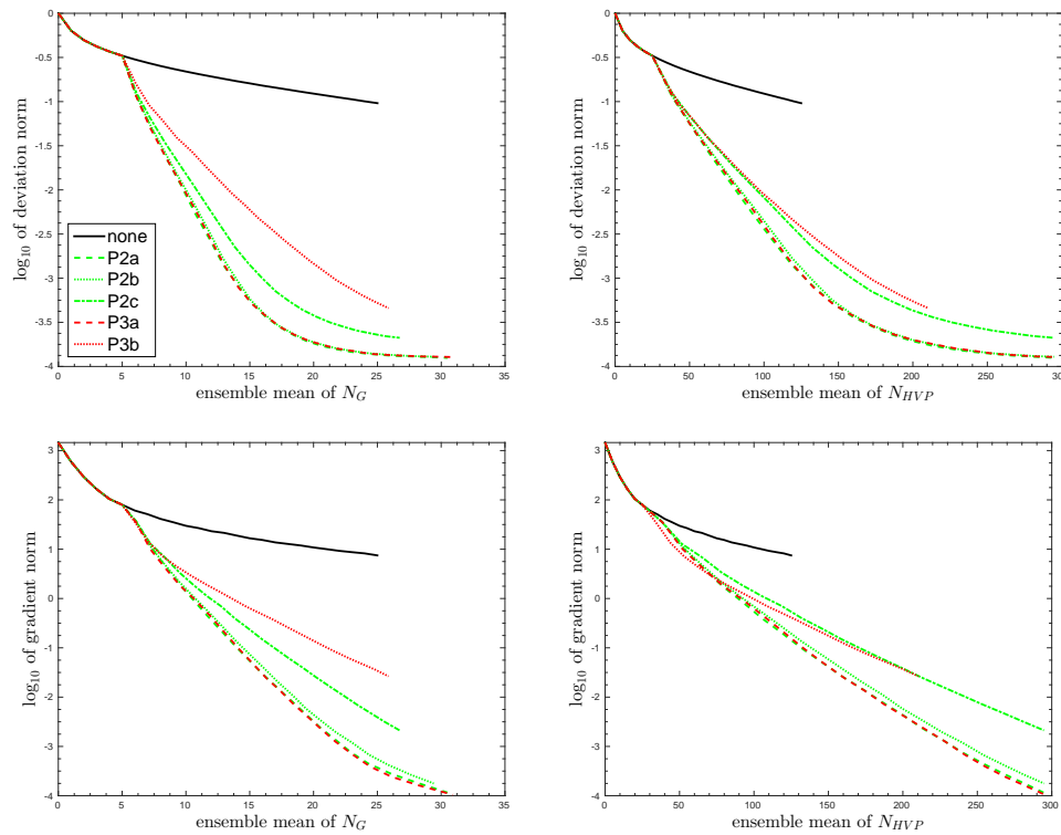
FIG. 5.8. Convergence diagram for MP3.
