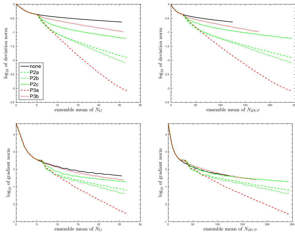
FIG. 5.7. Convergence diagram for MP2.
