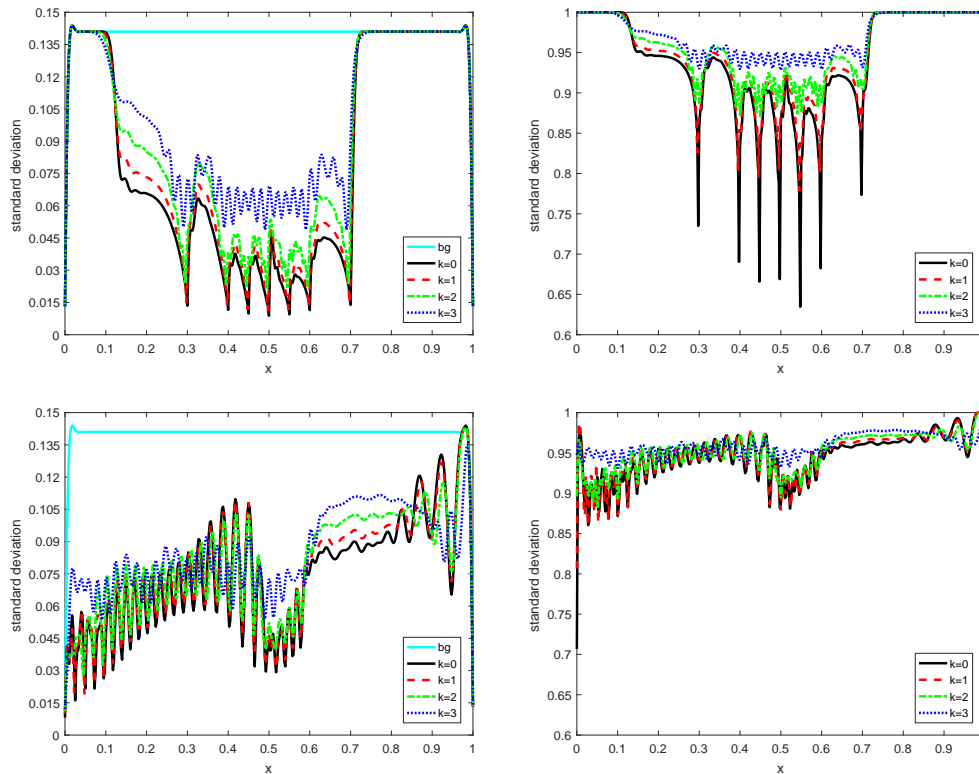
FIG. 5.3. Standard deviation before (left) and after (right) first-level preconditioning is applied. The top plots correspond to MP1 (stationary sensors), and the bottom plots to MP3 (moving sensor).
