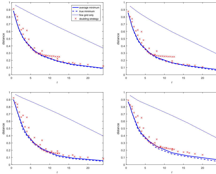
FIG. 5.5. Distance D (5.4) plotted against memory ratio r for model problems MP1 (top left), MP2 (top right), MP3 (bottom left) and MP4 (bottom right).
