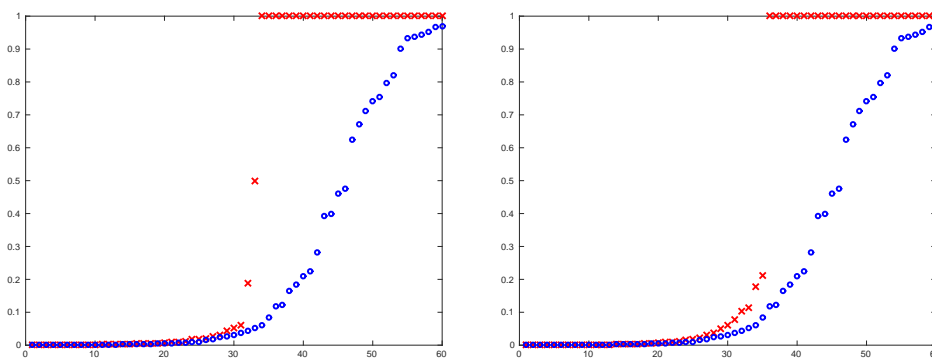
FIG. 5.4. A comparison of eigenvalues of H^{-1} (blue circles) and \tilde{H}^{-1} (red crosses) for two different eigenvalue combinations for MP1. Left: N_e = (0, 6, 13, 14) , D = 3.95e - 1 . Right: N_e = (0, 0, 29, 6) , D = 3.39e - 1 .
