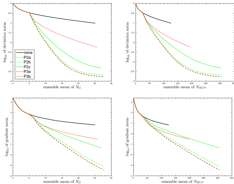
FIG. 5.9. Convergence diagram for MP4.
