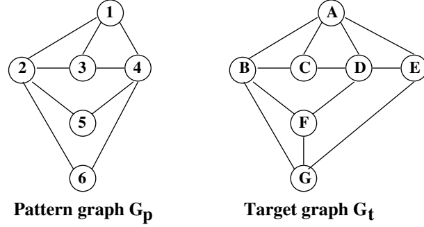
Fig. 1. Instance of subgraph isomorphism problem.
