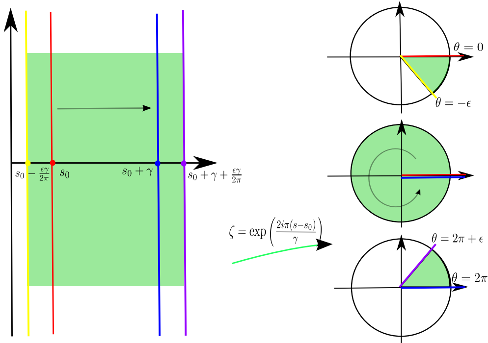
Figure 1: Holomorphic change of coordinates sends the green strip s_0 - \frac{\varepsilon\gamma}{2\pi} < \Re e(s) < s_0 + \gamma + \frac{\varepsilon\gamma}{2\pi} (Left) into the green subdomain D(\varepsilon) (Right) of the Riemann surface associated to the logarithmic function.
