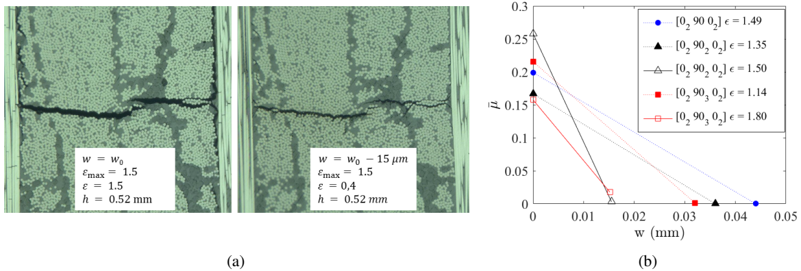
Figure 8. Micro-delamination length \bar{\mu} measured on the edge of the specimen at the surface ( w = w_0 ) and through the width w , 8(a): Micrographs before and after removing 15 \mu m of the width, lay-up: [0_2/90_2/0_2] , 8(b): Evolution of delamination density according to polishing depth (maximal applied strain \varepsilon in %).
