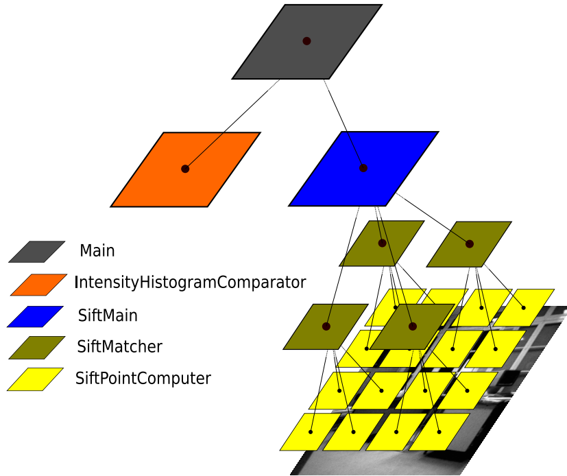
Fig. 1. Our architecture for object matching. At the lowest level, 16 SiftPointComputer agents extract SIFT points from the image and send them to their SiftMatcher parent. SiftMatcher agents then look for the closest SIFT point in the object database. SIFT matches are then handled by the SiftMain agent, which clusters them into compatible object pose hypotheses and send top-down predictions for future SIFT matches. The Main agent gathers SIFT evidence for an object presence, requests top-down histogram analyses from the IntensityHistogramComparator agent, and finally takes decisions.
