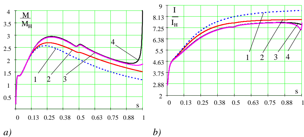
Fig. 5. Mechanical starting (a) and electromechanical (b) characteristic of SDSZ-20-29-54-80-UHL4 motor: 1 is naturally occurring characteristic; 2, 3, 4 are simulated ones for C = 4, 12, 7 and 14 \mu\text{F} respectively.
