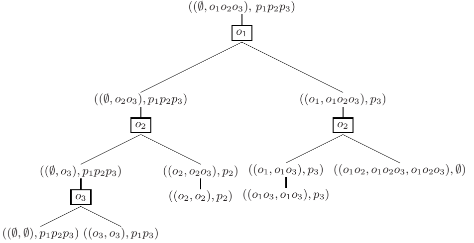
Fig. 3. Formal concept extraction on \mathbf{r}_5
