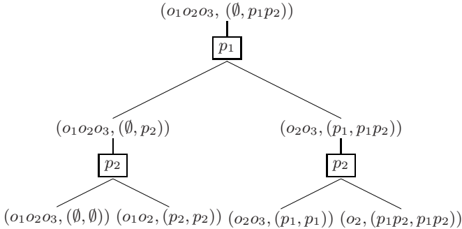
Fig. 2. Formal concept extraction on \mathbf{r}_4
