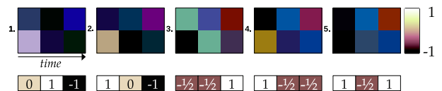
Figure 3: Five examples of CNN filters that seem to perform derivation
