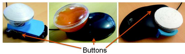
Figure 8: Different versions of the (A←B) compound device, from left to right: based on a 3D printed support (prototype v2), carved on the center of the mouse (prototype v3a) and carved on the right side of the mouse (prototype v3b)
