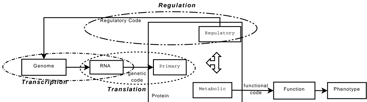
Figure 5: Overview of all the protein roles in the model. Proteins play different roles depending on the elements they interact with. They are translated from the genome (actually from mRNA); they can regulate mRNA transcription in addition to contributing to the phenotype.
