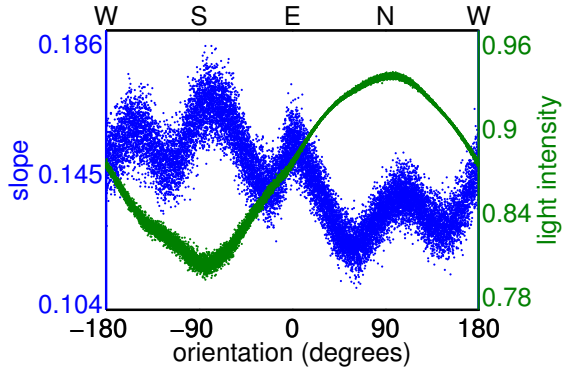
FIGURE 7 – Variation of slope (blue) and light intensity (green) with orientation. The slope is systematically larger on the southern sides of valleys, where the light intensity is lower. The secondary structure in the dependence of slope on orientation reflects tendency of valleys to grow in the cardinal directions, as seen in figure 1. Each point represents the average of 1000 points from the topography.
