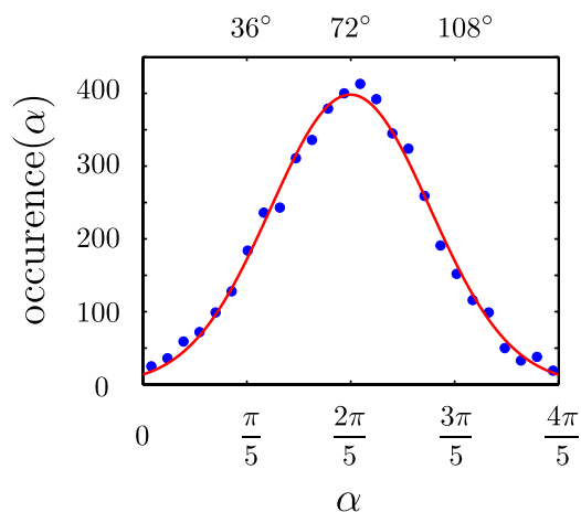
Fig. 6. Histogram of 4,966 measured junctions (blue points), compared with a Gaussian distribution (red) with the sample mean and variance. The estimated mean bifurcation angle, \langle \alpha \rangle = 71.9^\circ \pm 0.8^\circ , is consistent with the prediction \alpha = 2\pi/5 = 72^\circ .
