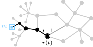
Figure 3: Monitor m sends a packet to destination address t on an unallocated port; the node r(t) answers with an error packet with source address i , and thus m discovers interface i of r(t) .
