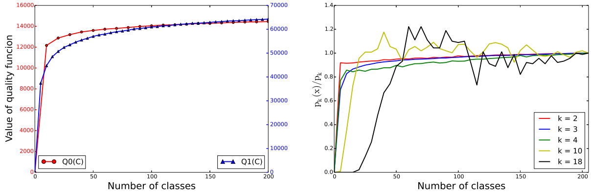
Figure 12: Left: evolution of the quality of the monitor set when we add colocation classes. Right: ratio of the observed fraction p_k(x) of routers of degree k with x colocation classes over the final obtained value p_k (with all classes).
