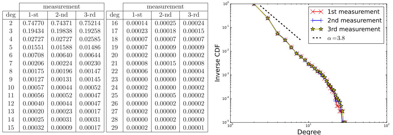
Figure 5: Left: the degree distributions obtained from our three measurements (after bias correction): for each degree k , we give the estimated fraction p_k of core routers with degree k . Right: plot of the inverse cumulative degree distributions obtained from our three measurements, after bias correction: for each value x on the horizontal axis, we plot the fraction of core routers having degree higher than or equal to x (log-log scale). We also plot the power law of exponent \alpha = 3.8 to show that obtained distributions are incompatible with a power law of exponent lower than this.
