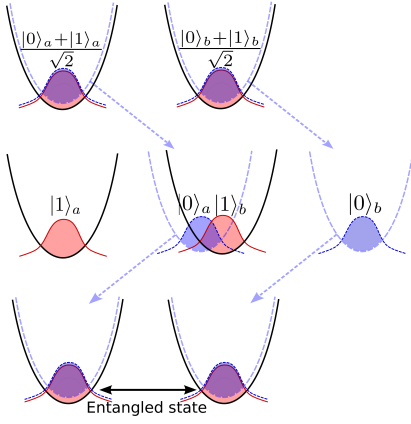
FIG. 1: (Color online) Sequence allowing to entangle condensate a (left well) and b (right well) via controlled collisional interaction in state dependent trapping potentials. The interaction phase, where the correlations are created, is depicted in the central panel.
