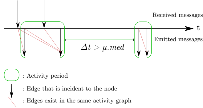
Fig. 1. For a node, the messages that are emitted are grouped into activity periods. The set of incident edges forms activity graphs.
