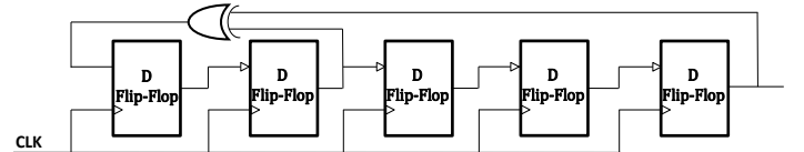
Fig. 1 Structure of the 5-bits PRNG
