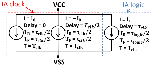
Fig. 7. Internal Activity of the core block
