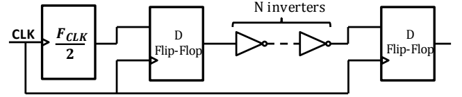
Fig. 5. Structure of a delay line
