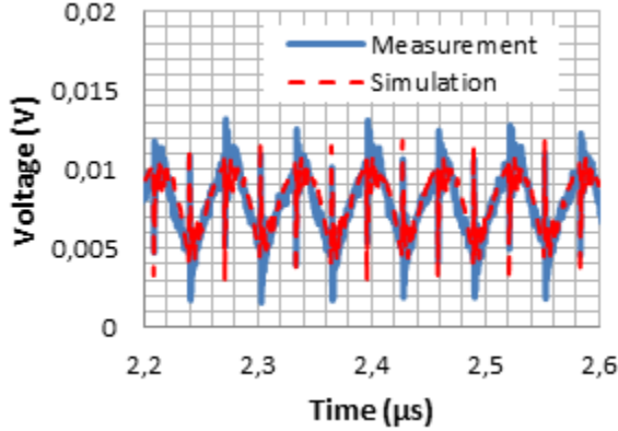
Fig. 8. Comparison between the measured and simulated external voltage using a 1 \Omega probe in the time domain
