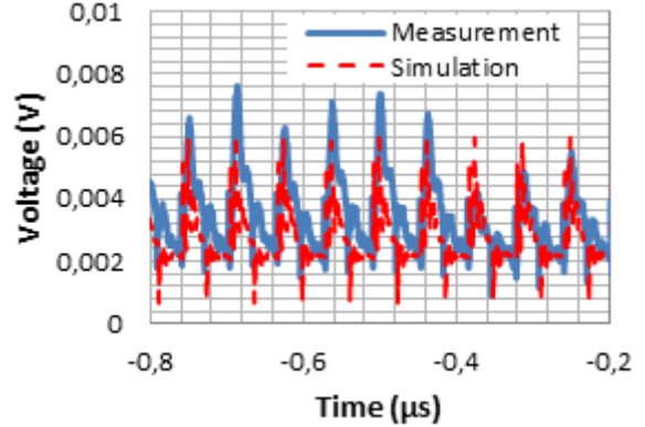
Fig. 10. Comparison between the measured and simulated external voltage using a 1 \Omega probe in the time domain
