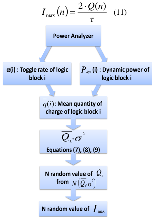
Fig. 4. Workflow of the IA construction using the statistical approach
