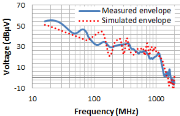
Fig. 13. Comparison between the measured and simulated external voltage using a 1 \Omega probe in the frequency domain
