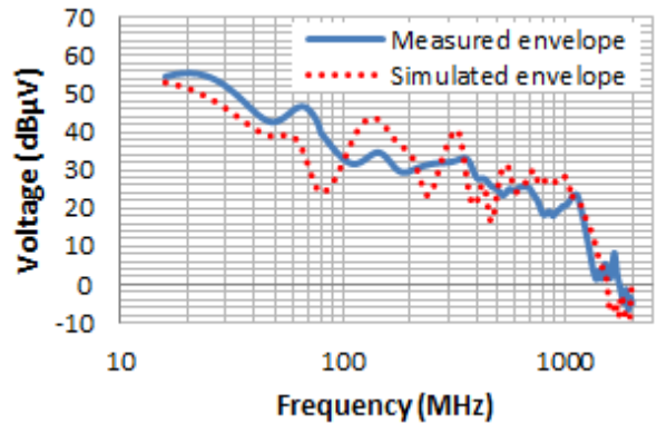
Fig. 11. Comparison between the measured and simulated external voltage using a 1 \Omega probe in the frequency domain
