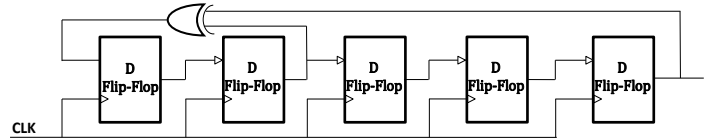
Fig. 1 Structure of the 5-bits PRNG
