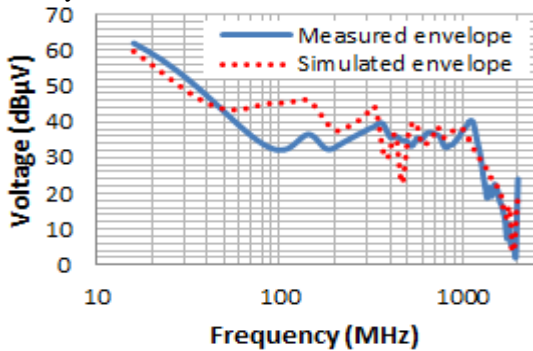
Fig. 9. Comparison between the measured and simulated external voltage using a 1 \Omega probe in the frequency domain
