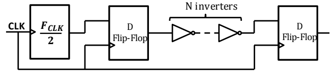
Fig. 5. Structure of a delay line
