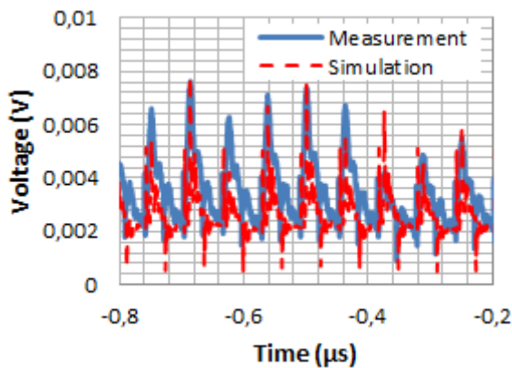
Fig. 12. Comparison between the measured and simulated external voltage using a 1 \Omega probe in the time domain
