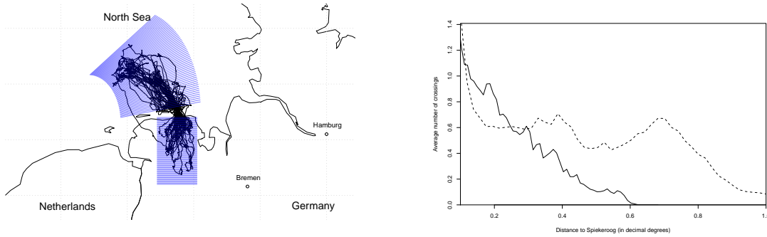
Figure 12: Lesser black-backed gulls' trajectories with the two sets of crossings segments S_{\text{sea}} and S_{\text{inland}} (left) and average number of crossings of a daily bird's trajectory in the sea direction (dashed line) and inland direction (solid line) with respect to the distance to Spiekerroog in decimal degrees (right).
