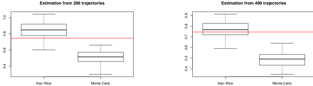
Figure 9: Boxplots over 100 replicates of Monte Carlo and non-stationary Kac-Rice estimators of C_{S_3}(20) for the two-dimensional telegraph process from n = 200 (left) and n = 400 (right) trajectories extracted from a temporal grid with step size h = 1 . The (spatial) integration step size is \Delta = 0.1 .
