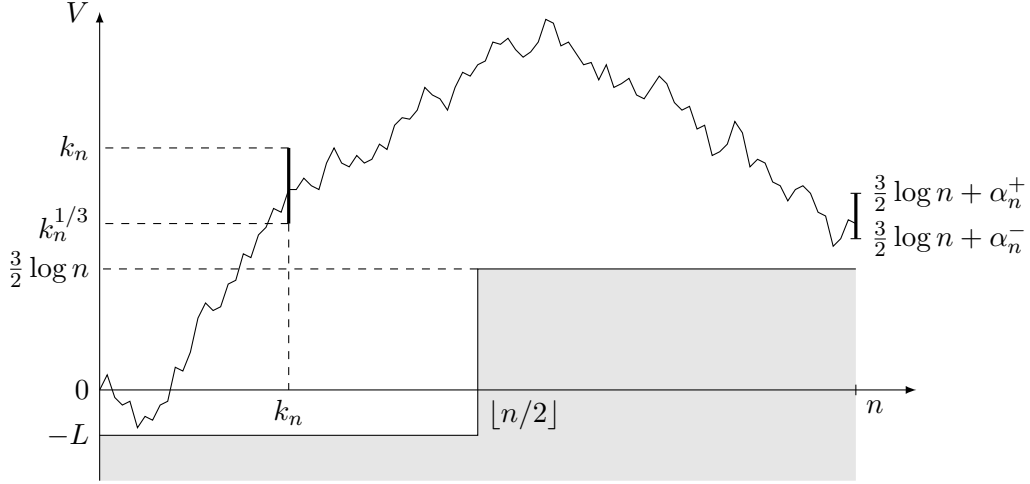
Figure 1 – Representation of the trajectory of a particle in A_n . It has to stay above the gray area and to pass through both thick segments.
