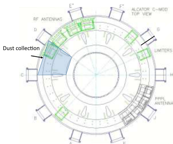
Fig. 1. Schematic of the Alcator C-Mod horizontal mid-plane showing 10 toroidal sectors corresponding to 10 lower outer divertor modules. Sectors are identified by the names: AB, BC... JK, KA. On the left side, the blue part shows where dust was collected in a given sector. (For interpretation of the references to color in this figure legend, the reader is referred to the web version of this article.)
