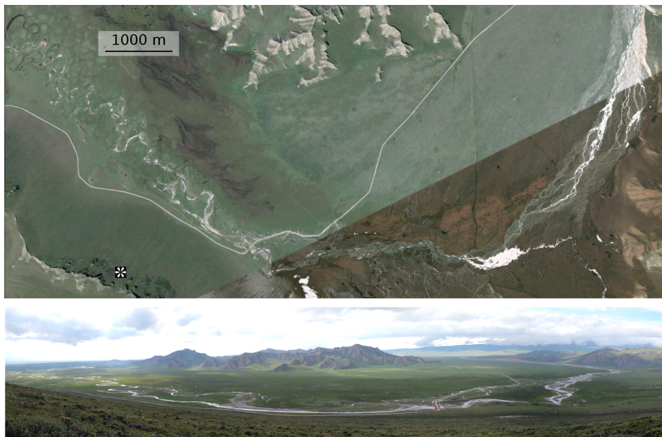
Figure 5. Satellite and panoramic view of a metamorphosis from braided to meandering (Bayanbulak Grassland, 84.578^{\circ} E, 42.721^{\circ} N, Google Earth). Marker on the satellite image indicates the viewpoint of the panoramic image. Its location also appears in Fig. 2.
