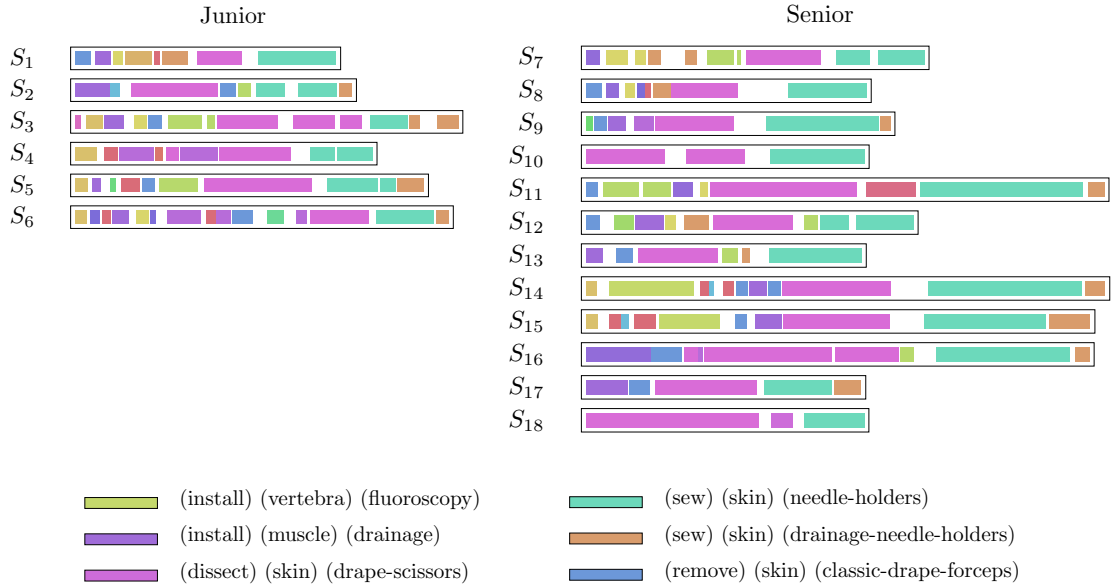
Figure 4: An extract of the second dataset of 18 ACD surgeries used for the experiments and the legend for the six most frequent actions.
