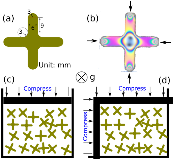
Figure 1. (a): Sketch of cross particle geometry. (b): Photo-elastic response generated by compressing a cross particle along each arm. (c): Schematic of uniaxial compression, using the bi-axial apparatus. (d): Sketch of biaxial compression. The gravity direction is given by \mathbf{g}
