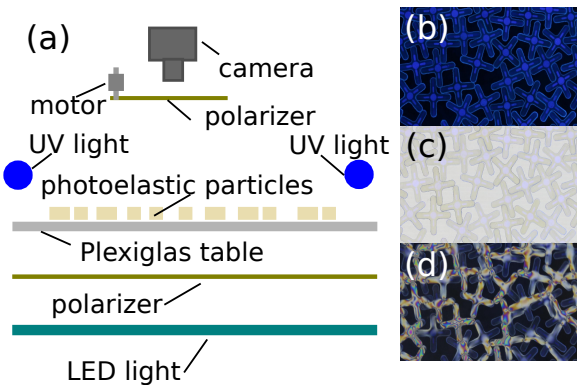
Figure 2. Experimental apparatus and typical experimental image data. (a): Schematic of the experimental apparatus, side view. Light from an LED source passes through a first circular polarizer, then through the transparent base of the apparatus and the particles. A stepper motor rotates a polarizer into or out of the line of sight of the camera, yielding polarized or non-polarized images. (b): Image with only UV light from above. Fluorescent bars on the arms yield the cross orientation. (c): Image with normal light and without the second polarizer. These images are used to detect particle positions. (d): Polarized image used to measure the pressure inside of the each particle.
