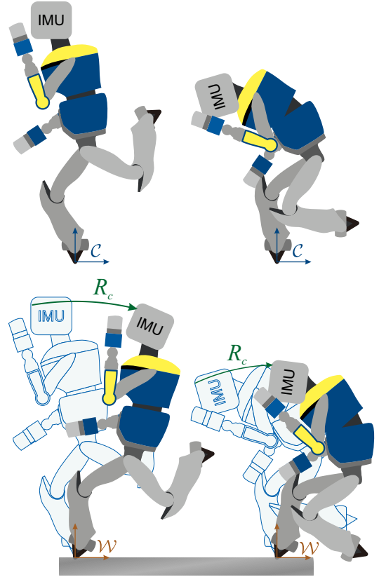
Fig. 1. Top figures: the robot is attached to the environment through a 3D pivot joint. The encoders only provide the configuration in a local frame called control frame and represented by \mathcal{C} . Bottom figures: In the world frame \mathcal{W} the configuration of the real robot is rotated compared to its value in the control frame (light wireframe robot). Only the IMU can provide data about this rotation, R_c . We need to account for encoders in this estimation, to distinguish local kinematics from pivot positions. For example the rotation R_c is here identical in the right and the left lower figures with different IMU configurations.
