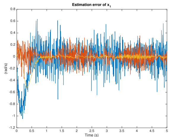
Fig. 3. Plot showing the estimation error for x_1 . On the top, the case where there is no noise, and on the bottom the noisy case. The colors blue, red, orange represent the three components of this vector respectively.
