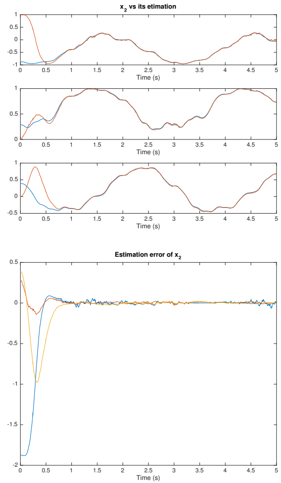
Fig. 5. Estimation of x_2 in the noisy case. On the top, three plots showing a comparison between respective components of x_2 in red and its estimation \hat{x}_2 in blue. On the bottom we see the evolution of the estimation error \tilde{x}_2 . The colors blue, red, orange represent the three components of this vector respectively.
