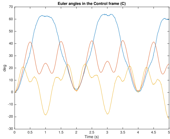
Fig. 2. Plot showing the values of the orientation of the IMU in the control frame ( \mathcal{C} ) expressed using Euler angles (blue: roll, red: pitch, orange: yaw)
