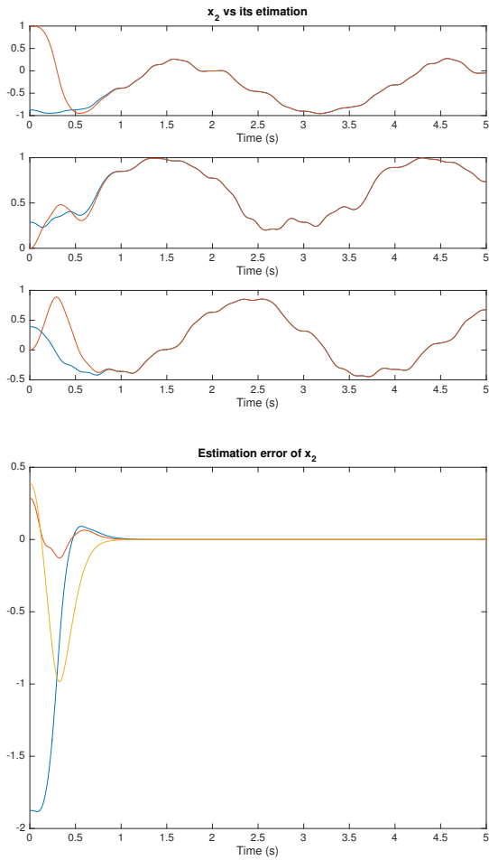
Fig. 4. Estimation of x_2 in the case without noise. On the top, three plots showing a comparison between respective components of x_2 in red and its estimation \hat{x}_2 in blue. On the bottom we see the evolution of the estimation error. The colors blue, red, orange represent the three components of this vector respectively.
