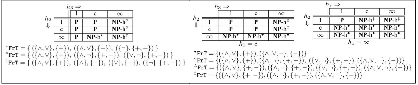
Figure 2: Summary of results: Individual decision-making (left) and egalitarian social welfare (right). Entries marked as “P” correspond to tractable settings (without any restriction). Instead, for the NP-hard scenarios, the tractability frontier is reported.
